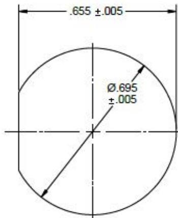
PANEL CUTOUT
